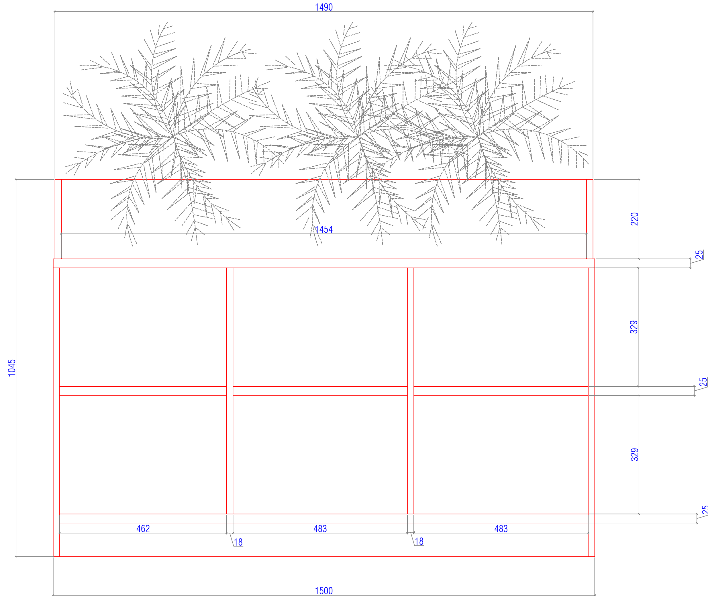
FRONT ELEVATION
