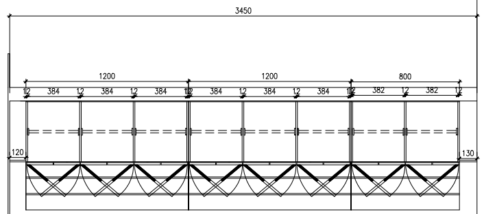
PLAN ( Z TYPE LOCKER WITH HPL STAND)
